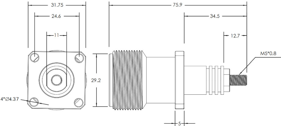
Dimensions are in mm
